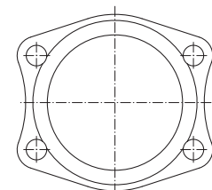
Flange as per SAE standard (Type GR-SAE)
