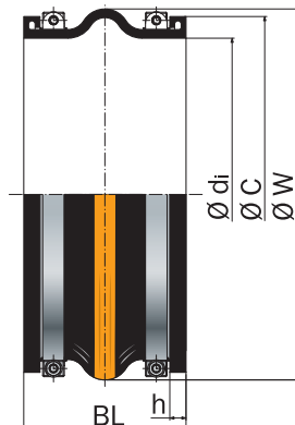
Type D-30 with tightening straps
