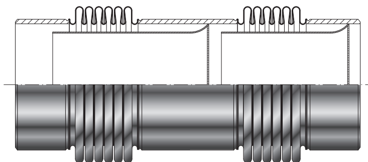
Type SA-23 with inner guide sleeve
