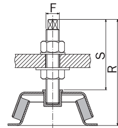
Type GMF-2 With male thread
