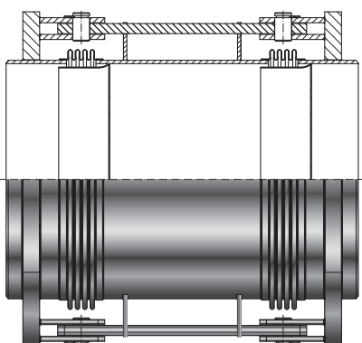
Type SA-24 with inner guide sleeve
