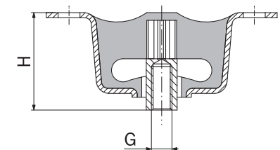
Type GMD-2 With female thread
