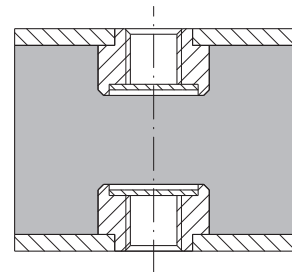
Type GMP-3 with female thread as per ISO 7-1
