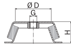
Type GMF-1 With female thread
