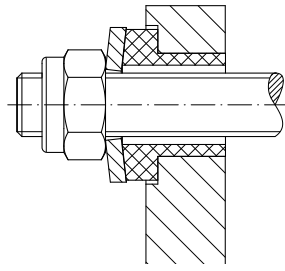
Sound-damping external restraint (lateral expansion joint)
