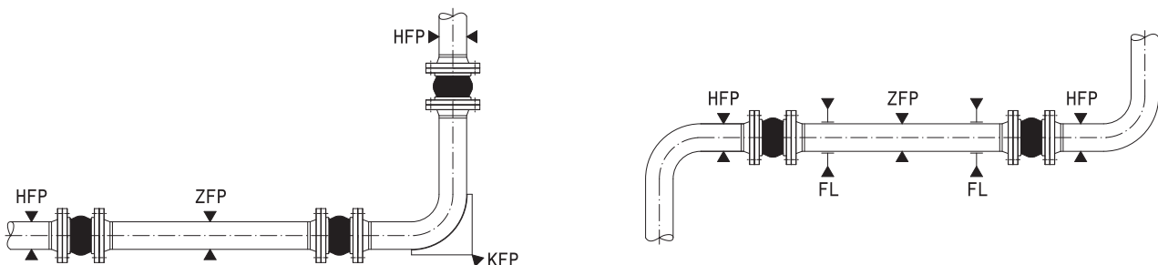
Fig. 4: Pendulum-type pipe suspensions are not fixed points
