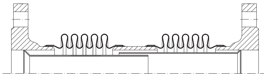
Axial expansion joint with telescopic guide sleeve
