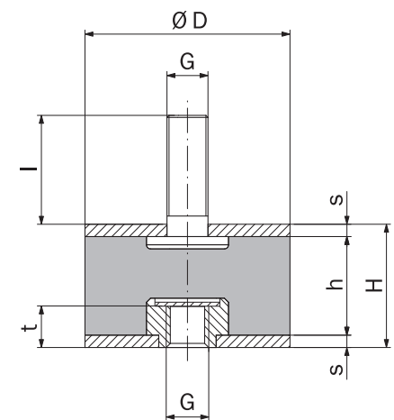
Type GMP-2 With male and female thread
