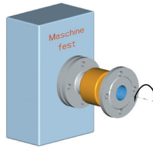
Type 11F Slow rotary movement with type 11F (1 fixed point, 1 side flexible)
