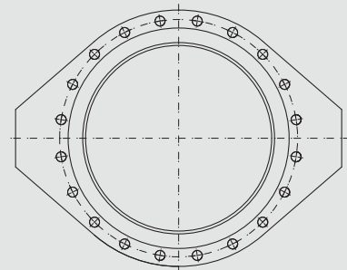
Oval flange (angular expansion joints)
