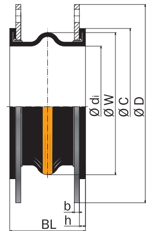
Type D-11 with flanges
