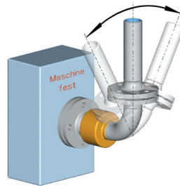
Type 12F Swivel movement with type 12F (1 fixed point, 1 side flexible)
