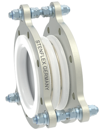
Type P-4 PTFE expansion joint
