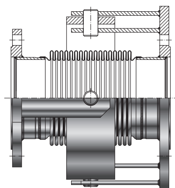
Type SF-33 with inner guide sleeve
