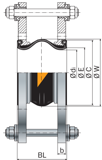
DN 25 - DN 150
